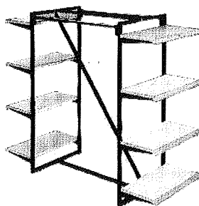
K411MAB Frame Only Rack Frame made of 1" Square Tubing with Matte Black Finish. 16 Shelf Brackets, 2-36" Chrome 1/4" Round Hangrails and Levelers. Shelves Sold Separately.
